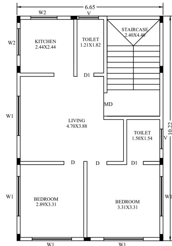
TYP: GROUND & FIRST FLOOR PLAN
