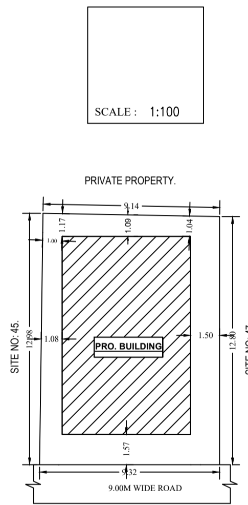
SITE PLAN
